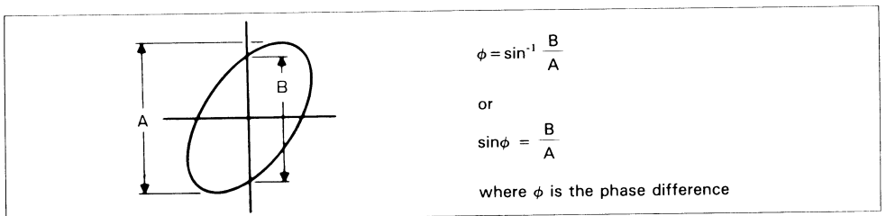
Figure 15. Measuring Phase Difference with Lissajous Patterns
