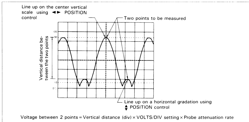
Figure 7. Measuring the Voltage Between Two Points
