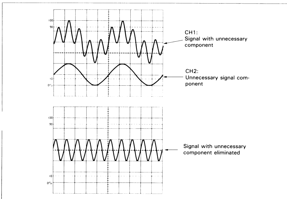
Figure 8. Common-Mode Rejection
