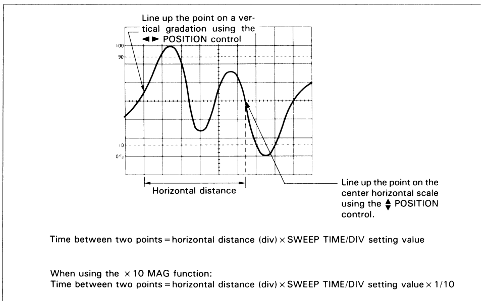
Figure 11. Time Measurement
