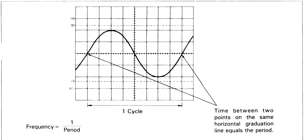
Figure 12. Measuring Frequency
