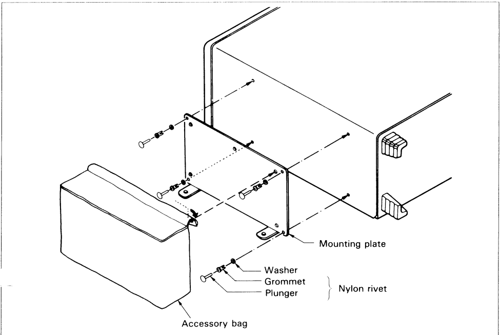
Figure 19. Attaching the Accessory Bag
