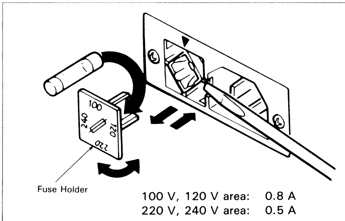
Figure 18. Fuse Replacement and Changing Voltage Requirements
