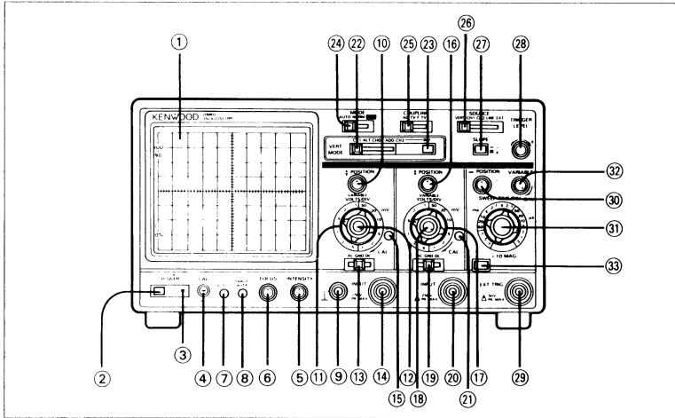
Figure 1. Front Panel
